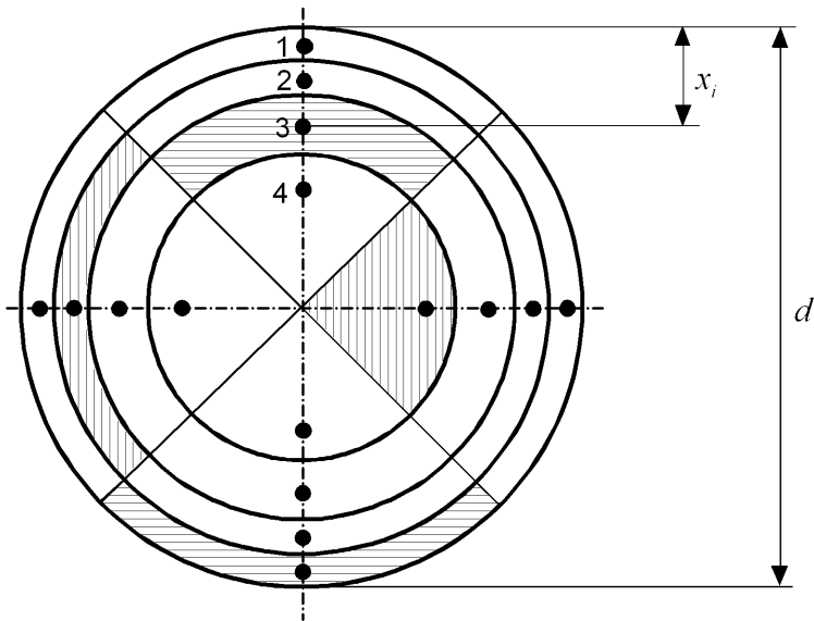
Figure C.2 — Sampling point positions in circular ducts - Tangential method (showing positions for ducts over 2 m diameter)
